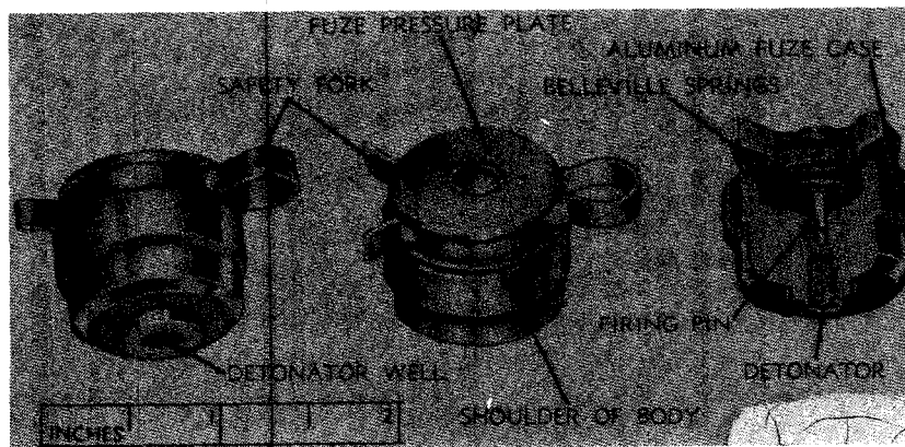
Fig 1-106 ANTITANK MINE FUZE, M603 (T17E2)
